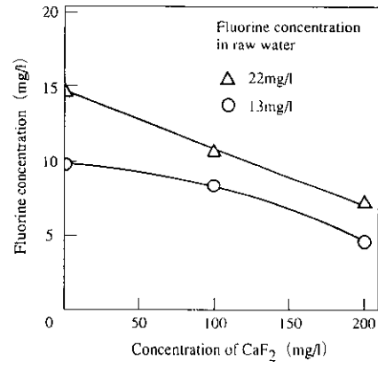
Fig. 4 Relationship between calcium fluoride concentration in flocculation-crystallization step and fluorine concentration in treated water by the sludge circulation system
