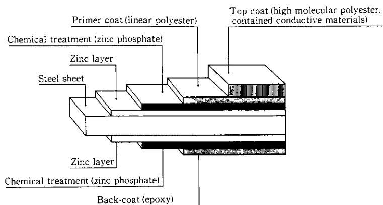
Fig. 2 Composition of the coating film
