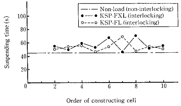
Fig. 3. Comparison of cell suspending time in construction
